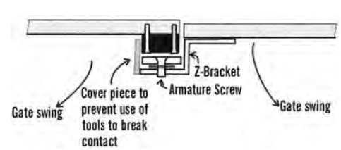
FIG. 3 - Installation on a double-swing gate
