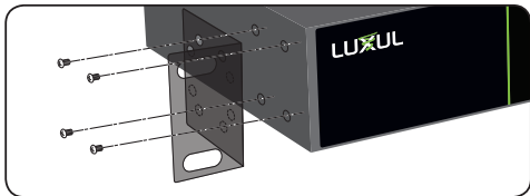
Rack-mounting the XMS-1208P
