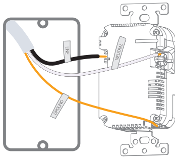
WIRING DIAGRAM
