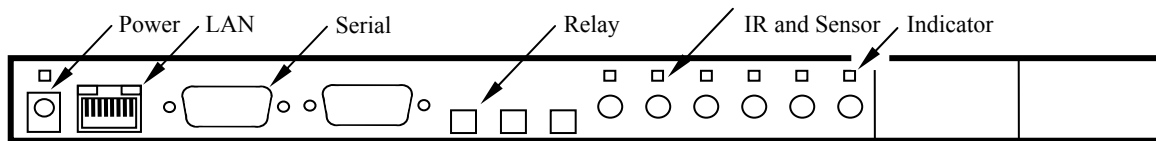
GC-100-12 Front Panel
