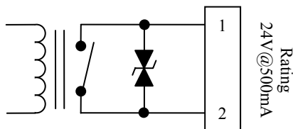
Relay Terminal Block Connector
