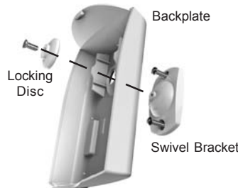
Figure 4. Swivel Mount Bracket
