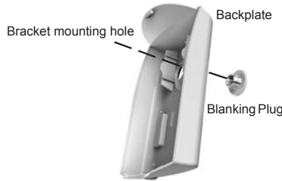
Figure 3. Prep for Wall Mounting (No Bracket)
