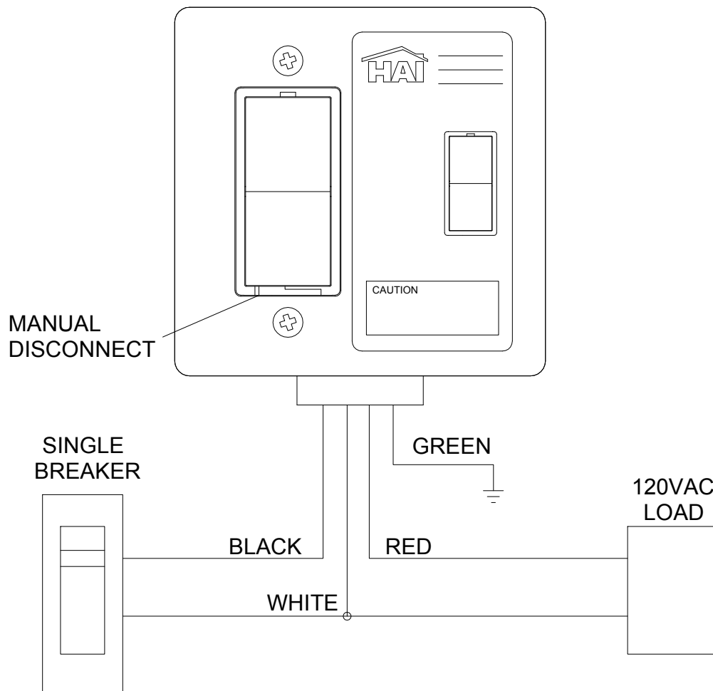
Figure 1 Connecting a 120VAC Device
