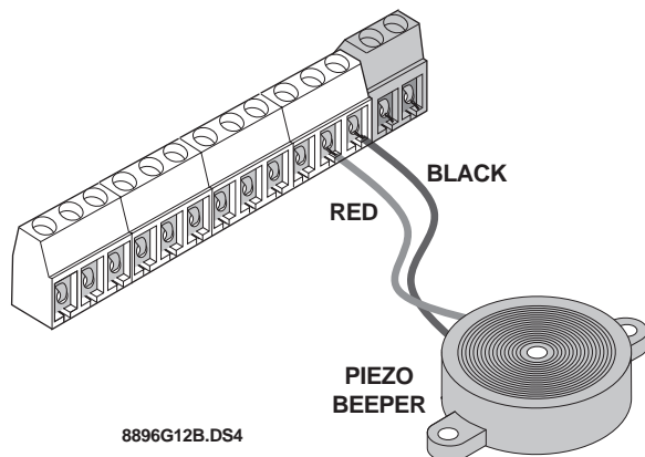
Figure 14. Piezo Status Beeper Connections
