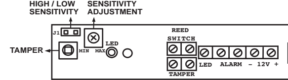
Figure 1B: Terminal Connections Diagram (RK600SMXX00A)
