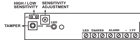
Figure 1B: Terminal Connections Diagram (RK600SMXX00A)
