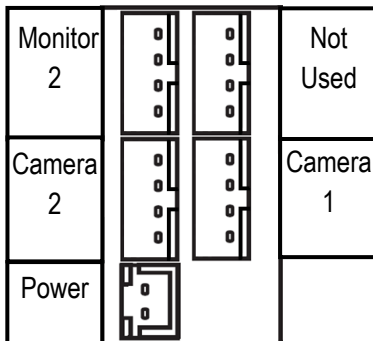
Figure 2 – Back of Primary Monitor Detail
