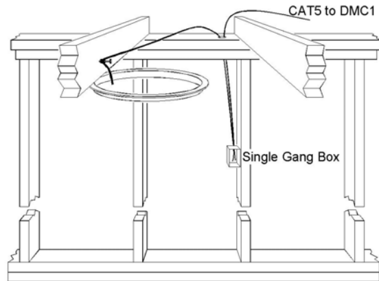
Figure 13 - Speaker installation
