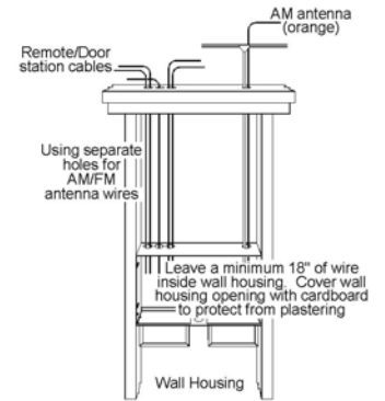
Figure 6 – Antenna installation
