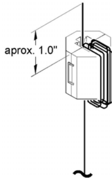
Figure 7 – Ferrite bead installation
