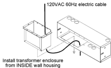
Figure 4 - Transformer placement
