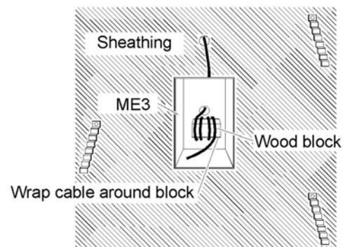
Figure 10 - ME3 installation
