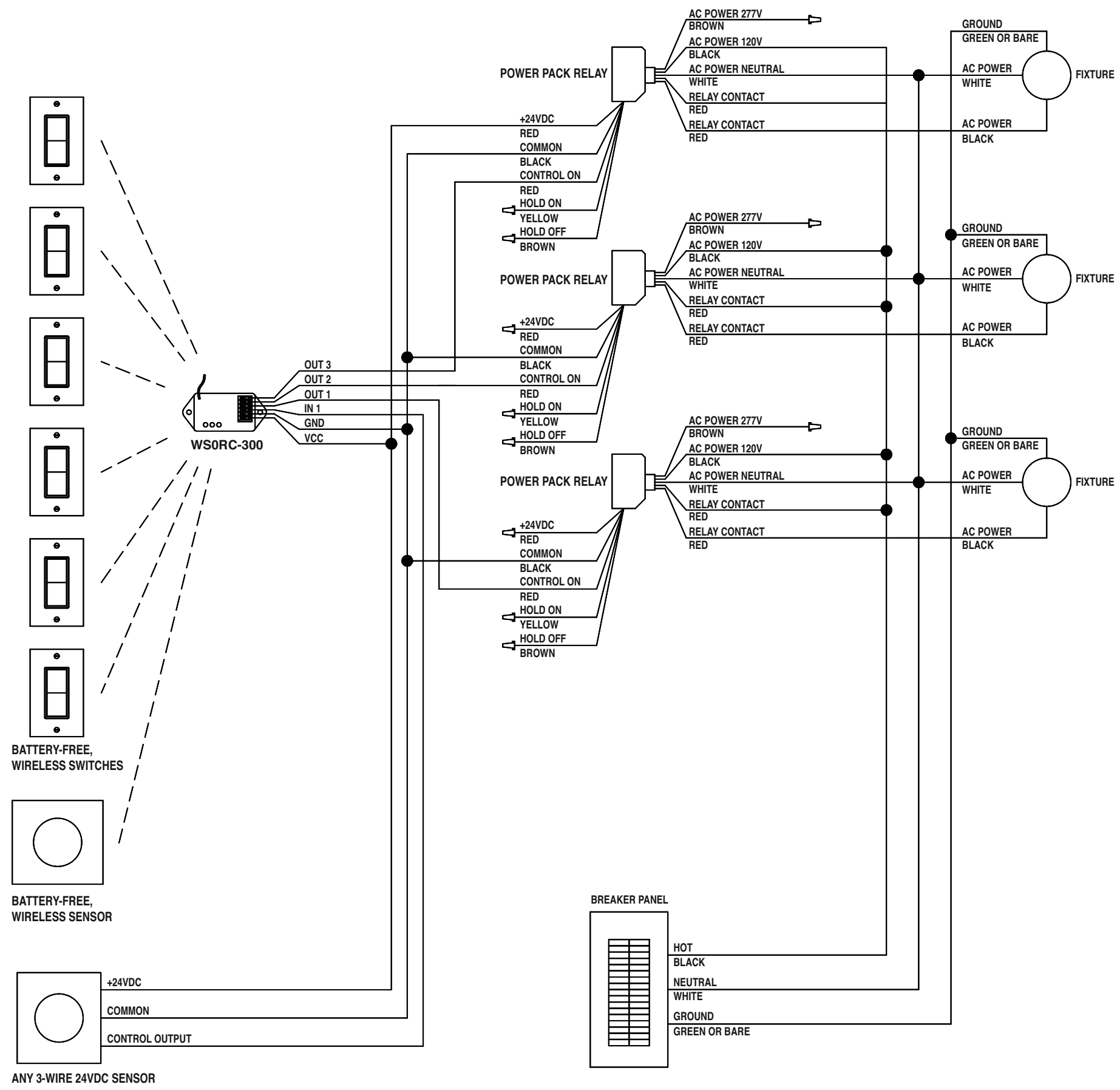
Figure A - Single Pole or Multi-way Wireless Switch (1 or more wireless light switches)
