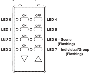
Figure 2 LED callouts for Non-Scene Operation, Individual Mode
