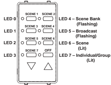
Figure 5 LED callouts in Scene Group Mode
